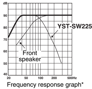
Frequency response graph*
