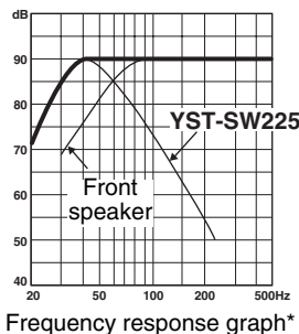
Frequency response graph*
